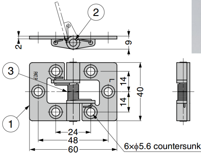
Above drawing is for GHG-BF3-2L-SC (GHG-BF3-2R-SC is symmetrical)
